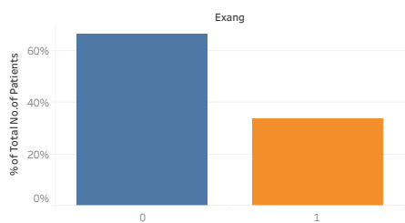
Exe-Ind-Angina
